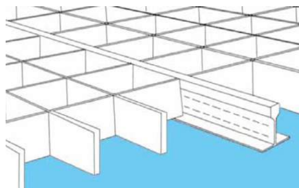
Capovolgere il pannello mm. 600x600 completo e assemblato Turn upside down the complete panel mm.600x600 assembled
