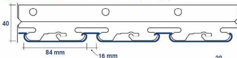
Type 63/Z STRONG main supporting carrier
