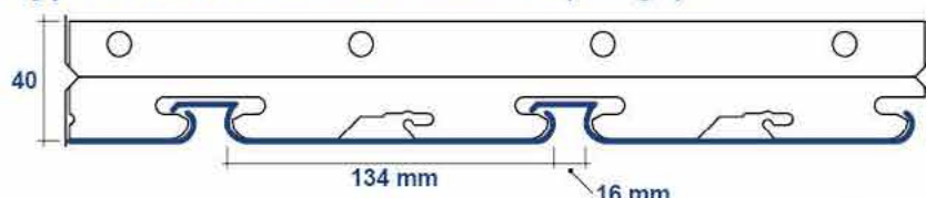
Type LT/150-R mm.134 + mm.16 open gap
