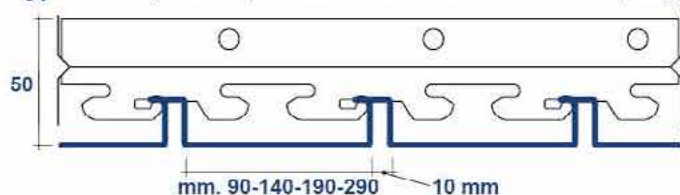
Type 63/Z STRONG main supporting carrier lenght mm.4000
